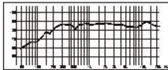
DSP255 II Freq. Response (dB SPL, 1W, 1m)
