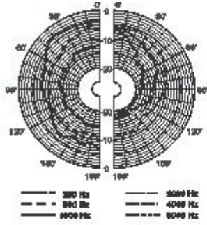
DSP255 II Vertical directivity pattern
